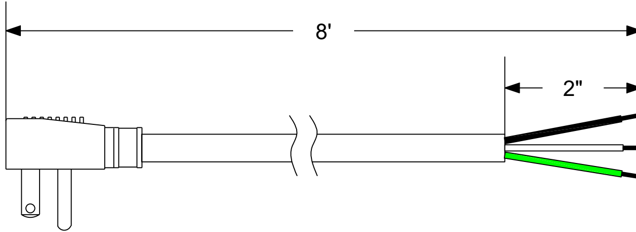
KK7000 NEMA 5-15P RIGHT ANGLE MOLDED
