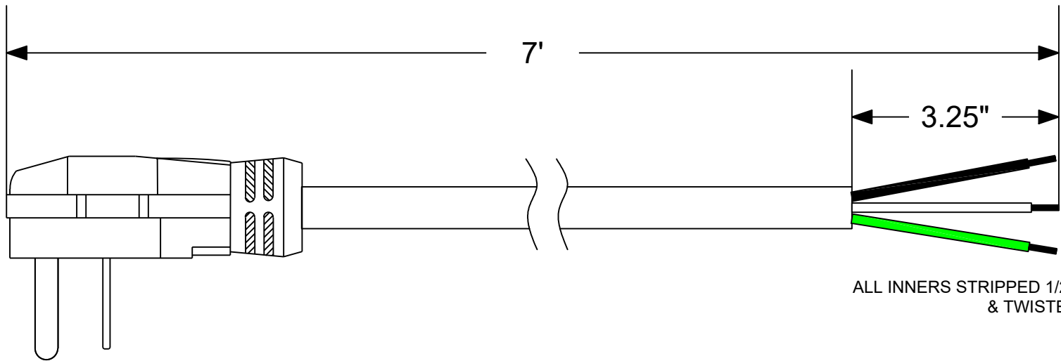
KK6-30P NEMA 6-30P RANGE PLUG MOLDED
